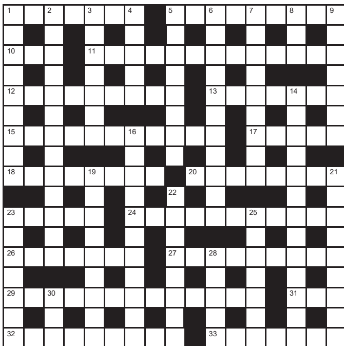
Solution Polymath 1,095
